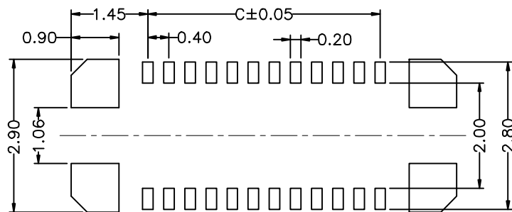
RECOMMENDED PCB LAYOUT CONNECTOR SIDE
